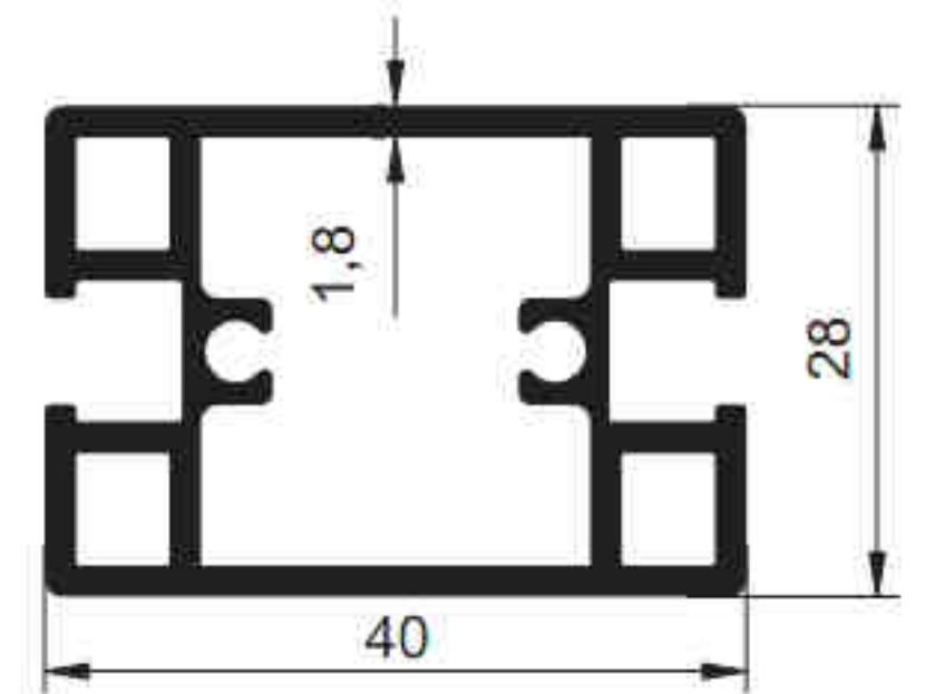
3663 - 0.954 kg/m
