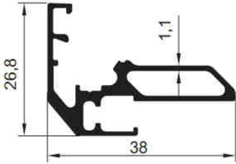
5340 - 0.461 kg/m
