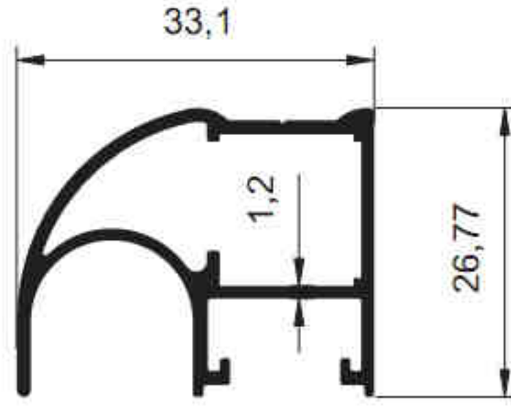
4451 - 0.447 kg/m
