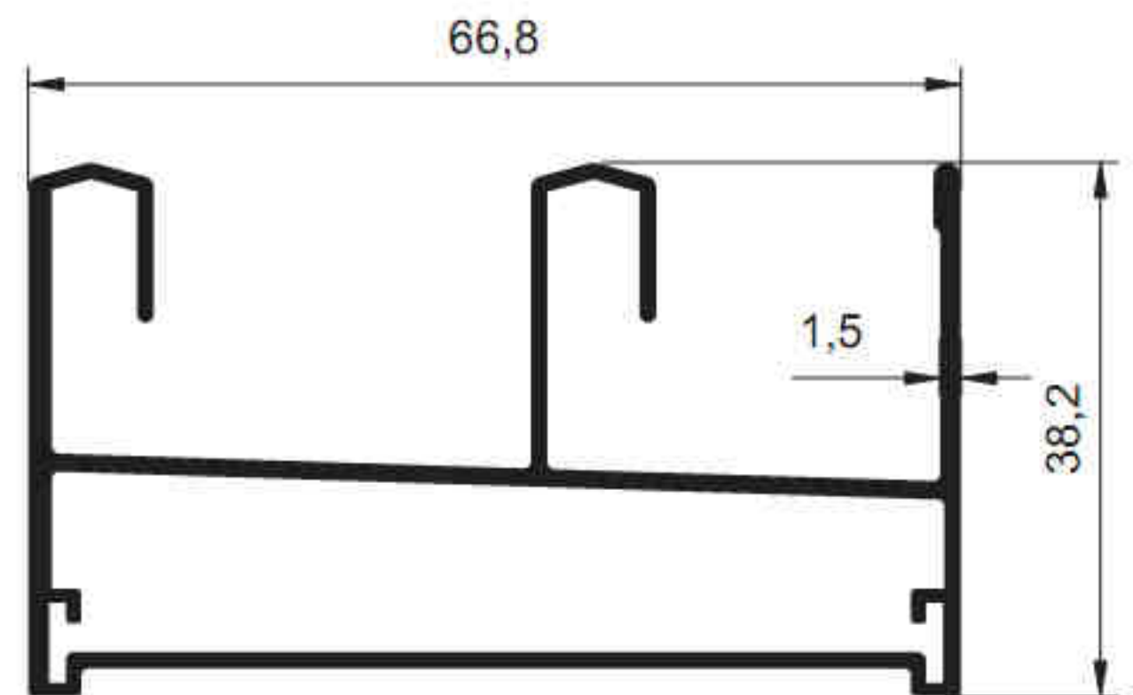
2203 - 0.957 kg/m
