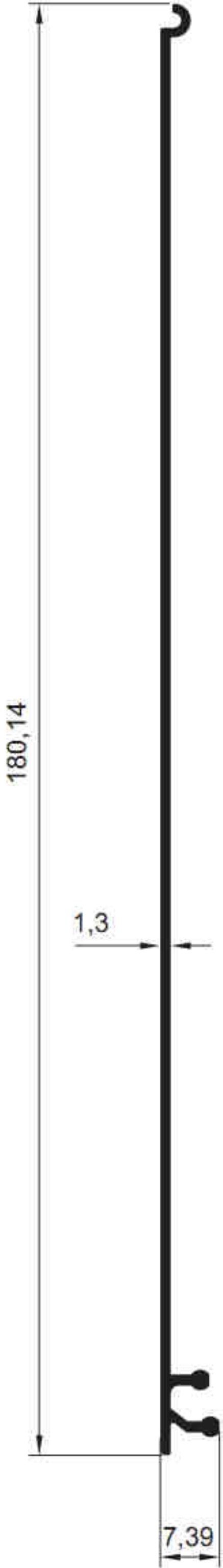
5580 - 0.691 kg/m
