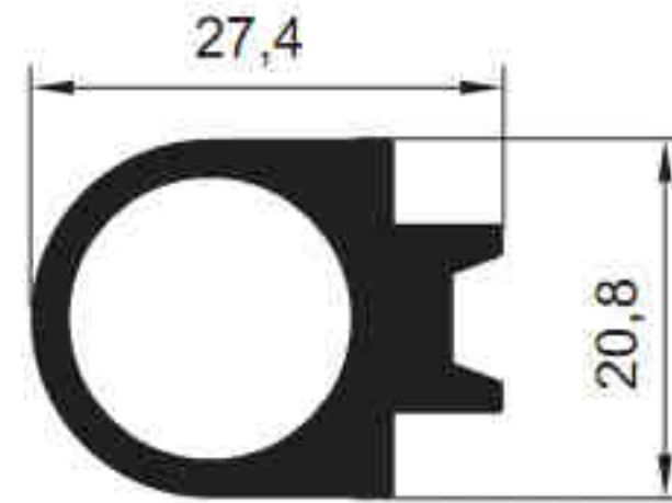
5559 - 0.635 kg/m
