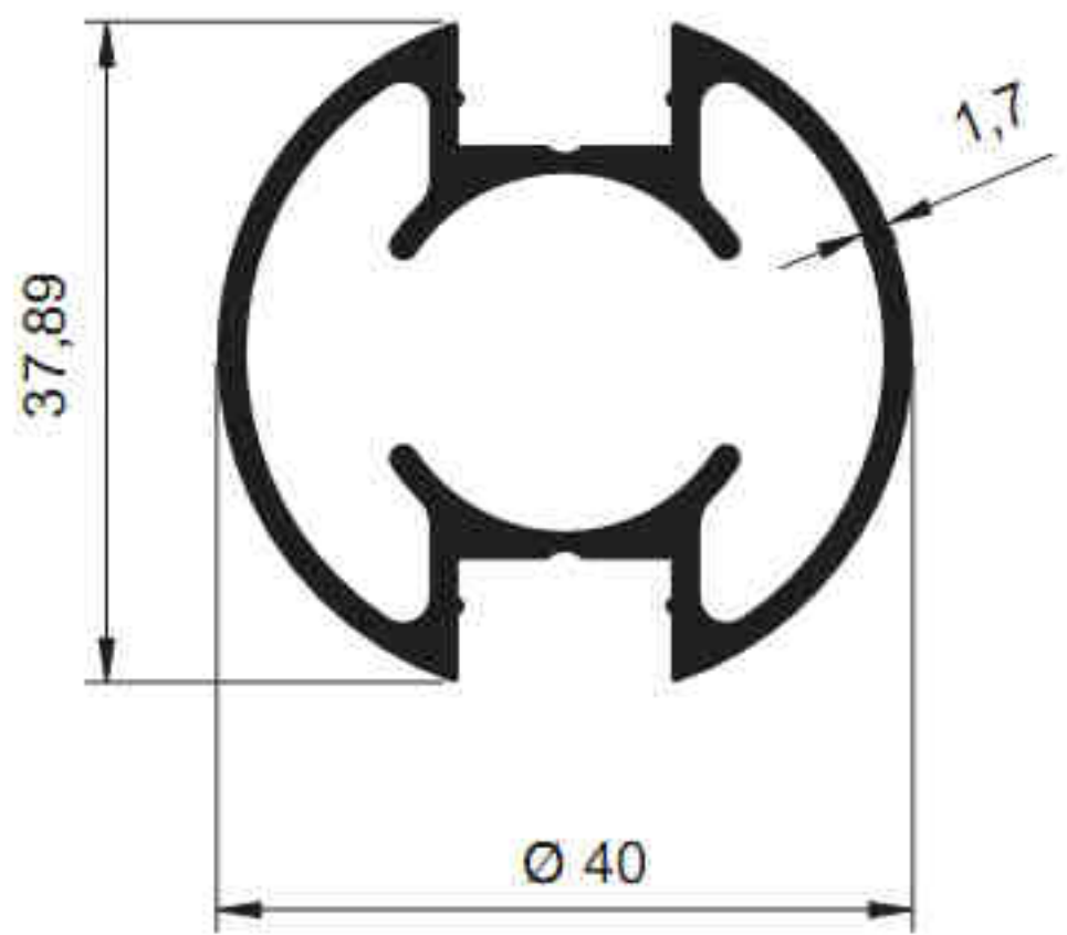
4981 - 0.835 kg/m
